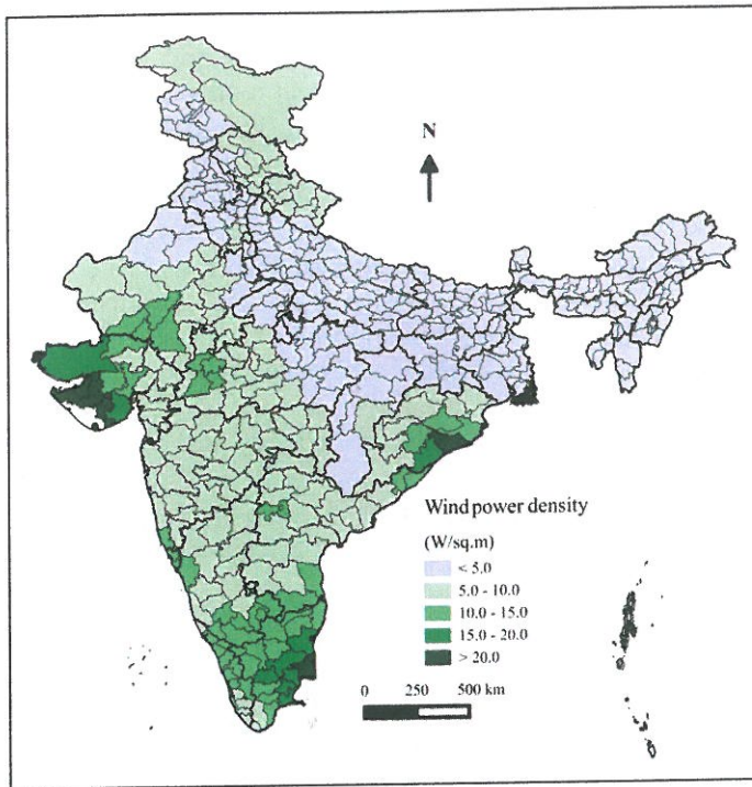
Fig. 15 District-wise wind power density potential in India
